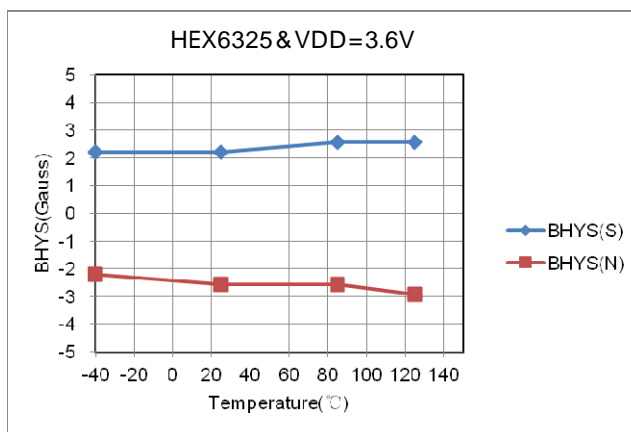
Hysteresis window versus Temperature (V DD =3.6V)
